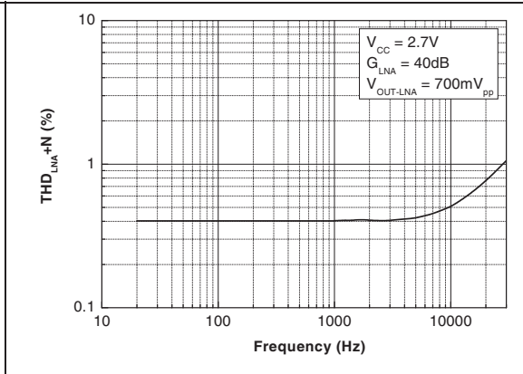
Figure 7. LNA distortion vs. frequency
