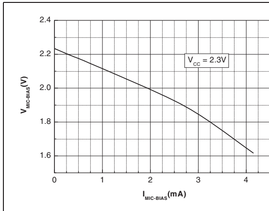
Figure 12. MIC-BIAS voltage vs. MC-BIAS current
