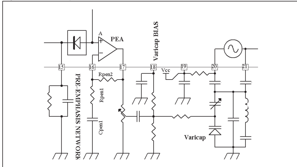
Figure 32. Pre-emphasis schematics
