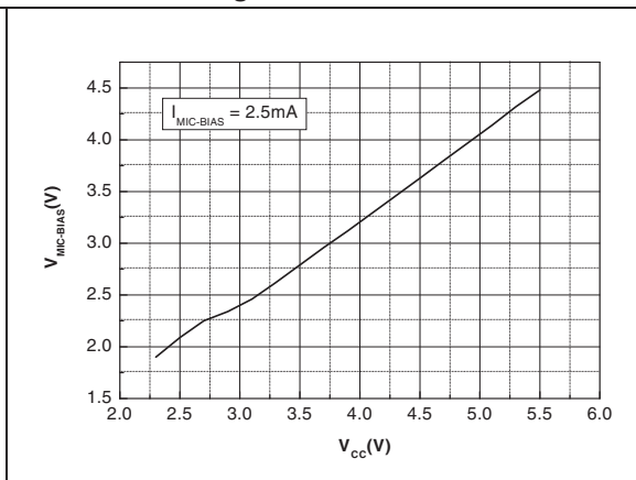
Figure 11. MIC-BIAS output voltage vs. supply voltage
